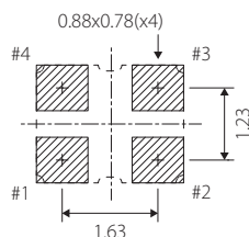
Land Pattern(REFERENCE)
